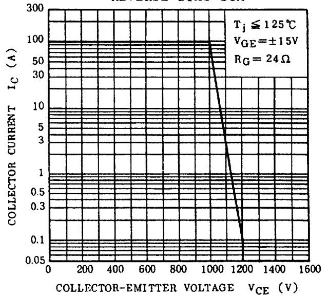
REVERSE BIAS SOA
